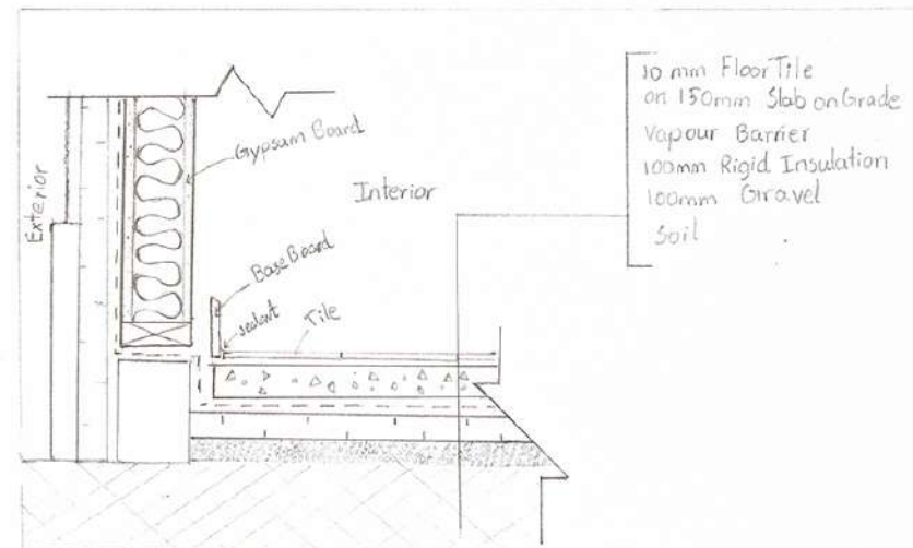
AD08 / Front-of-house floor at wall Scale / 1:20
